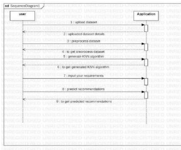
Fig4.2.3:Sequence diagram
