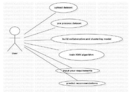
Fig4.2.1:Usecasediagram
